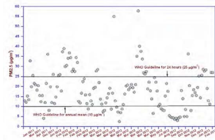
Figure 3-9: PM_{2.5} levels at MCOH from December 2010-February 2013. Adapted from: (Budhavant & Gustafsson, 2013).
