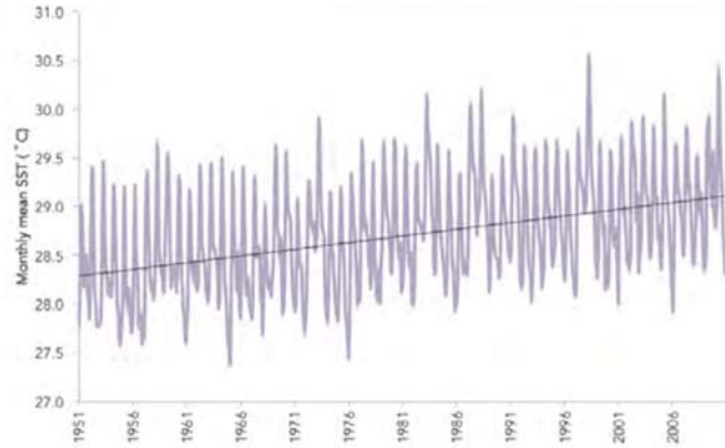
Figure 4-2: Sea surface trend in central Maldives from 1951 to 2010. Adapted from (MEE, 2015b)
